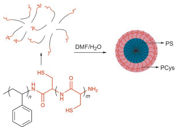
Figure 2. Steps in the self-assembly of poly(styrene- block -cysteine) (PS 100 PCys 20 ) conjugated block copolymer.
